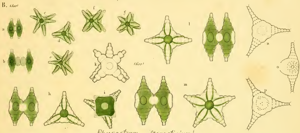
Phycostrium (Stenactinium)
