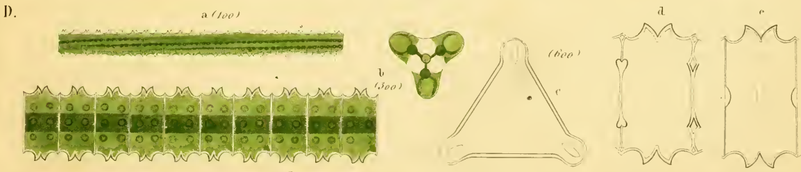
Desmidiium Swartzii.
