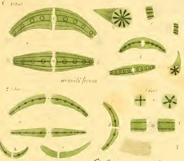
Closterium parvulum
